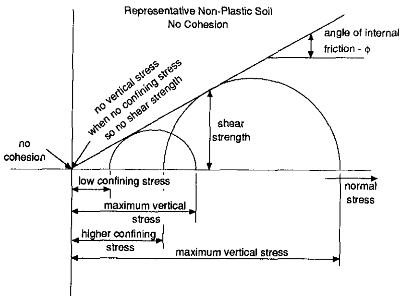
Fig. 12. Mohr's diagram for a nonplastic soil
