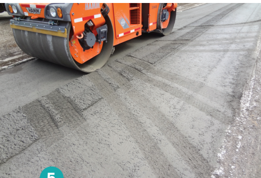
5 Even before rolling, driveways may be immediately reopened behind the paver if alternative access is not available
